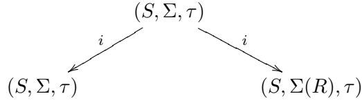
Figure 2: State bisimulation as a span.
