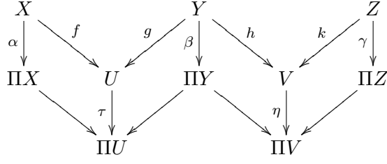
Figure 5: Composing cospans.
