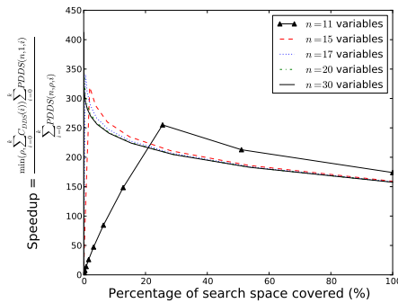
(c) Speedup of PDDS with \rho = 512 in function of the percentage of search space covered. Recalls C_{PDDS}(k) is the number of leaves processed at iteration k .
